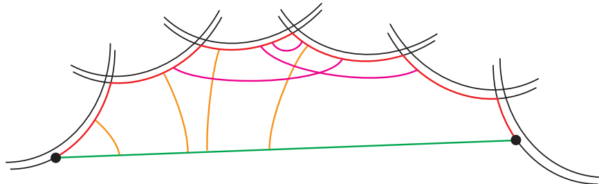
FIGURE 1. The diagram D , showing some possible (in orange) and impossible (in pink) dual curves.
