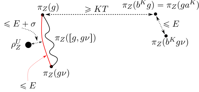
FIGURE 6. The arrangement of points in \mathcal{C}Z in the proof of Claim 1 in Case 4.
