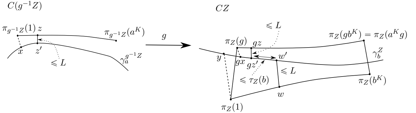
FIGURE 3. The geometry of the axes of a and b in \mathcal{C}g^{-1}Z and \mathcal{C}Z , respectively.
